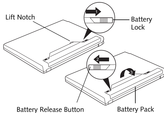
Figure 4-1. Removing a Battery
