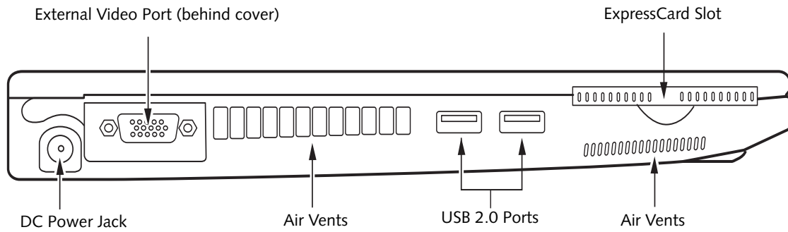
Figure 2-4. LifeBook notebook left-side panel
