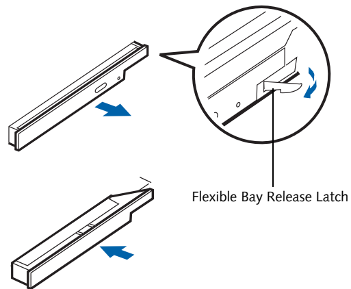
Figure 2-18 Removing/Installing a device in the Flexible Bay
