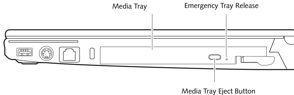
Figure 4-2. Optical Drive
