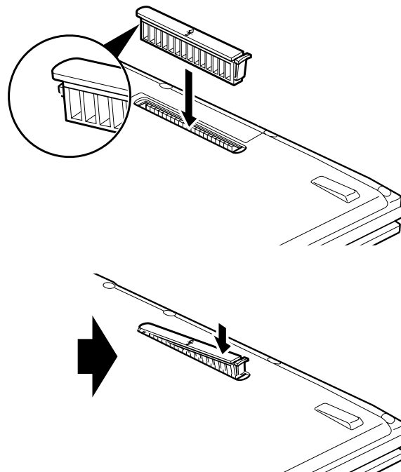
Figure 6-1 Removing/installing the dust filter
