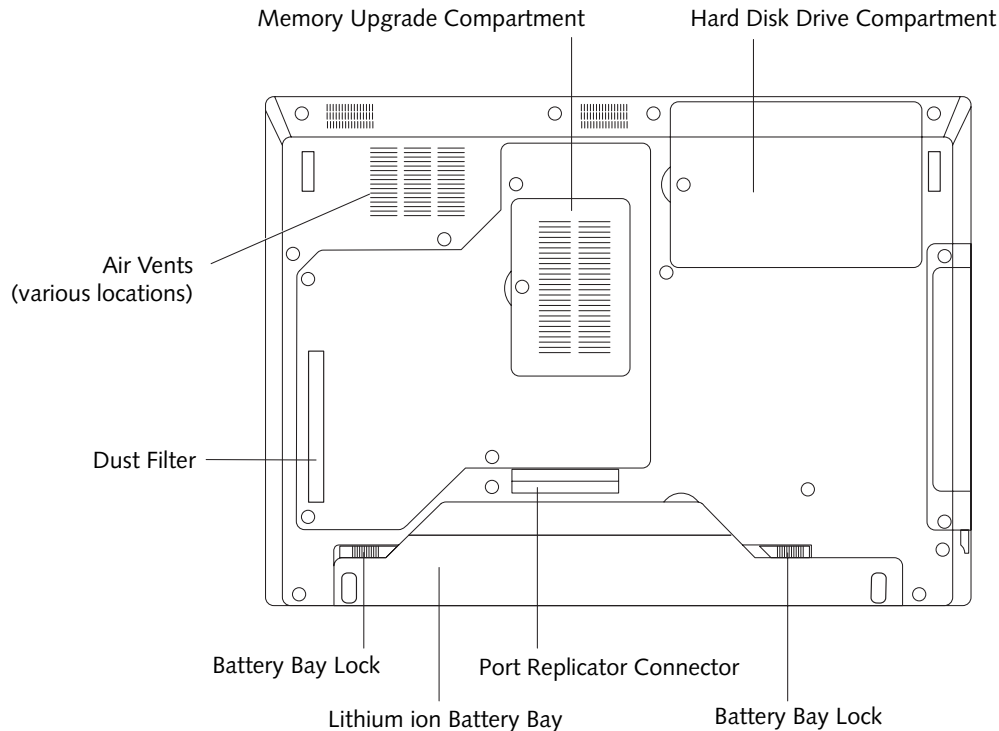
Figure 2-7. LifeBook notebook bottom panel
