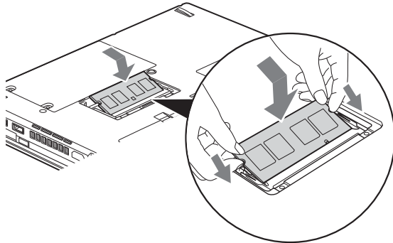
Figure 24. Inserting a Memory Module
