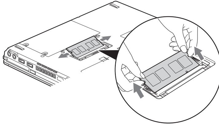
Figure 23. Removing a memory module
