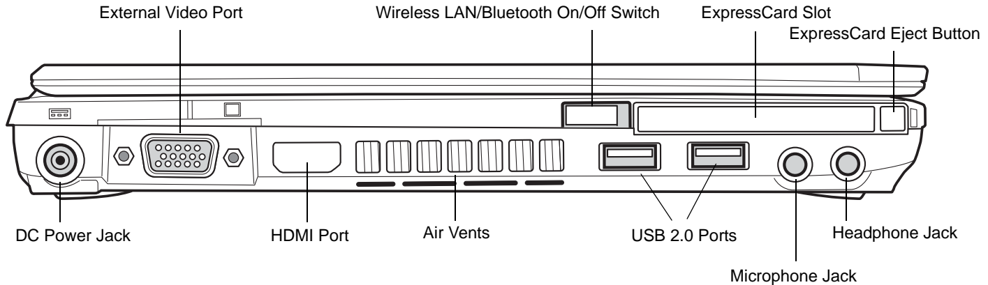
Figure 3. LifeBook notebook left-side panel
