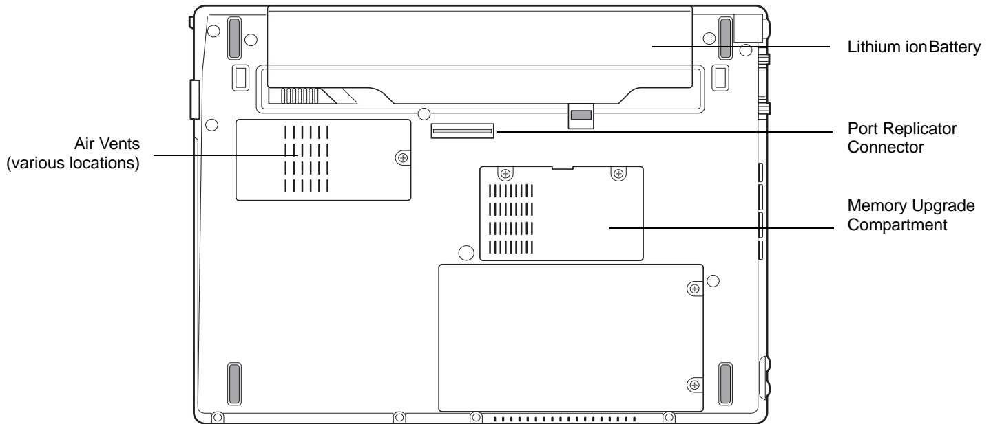
Figure 5. LifeBook notebook bottom panel
