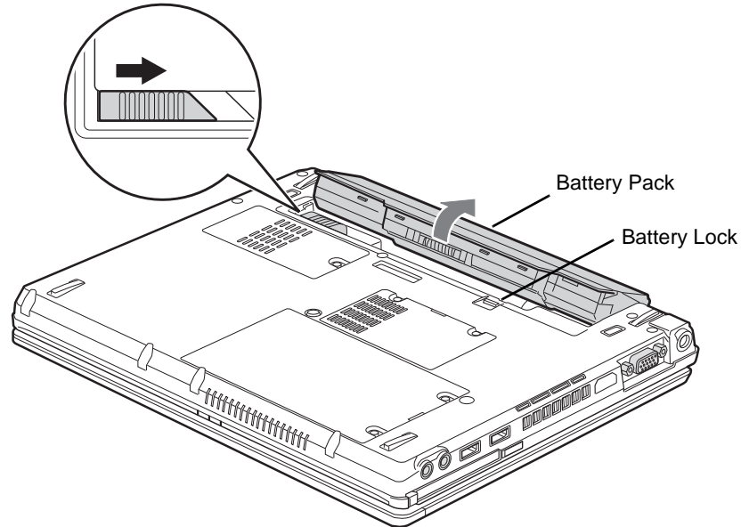
Figure 20. Removing the Battery
