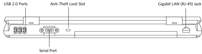
Figure 2-7. LifeBook notebook back panel
