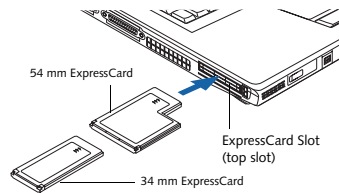
Figure 4-7. Installing/Removing ExpressCards
