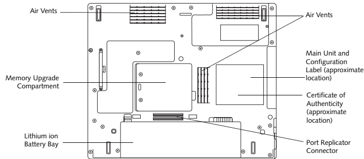
Figure 2-8. LifeBook notebook bottom panel
