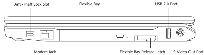
Figure 2-6. LifeBook notebook right-side panel
