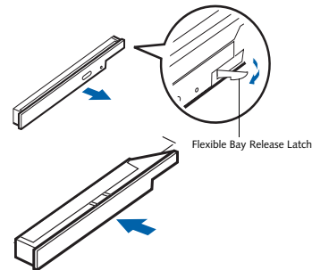
Figure 2-18 Removing/Installing a device in the Flexible Bay
