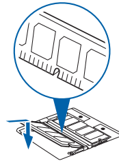
Figure 4-10. Installing a Second Memory Module
