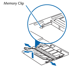
Figure 4-11. Removing a Memory Upgrade Module
