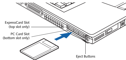
Figure 4-6. Installing/Removing PC Card
